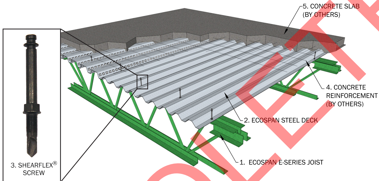
Figure 1-1: The Ecospan® Composite Floor System
