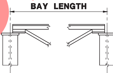
STEEL COLUMN
