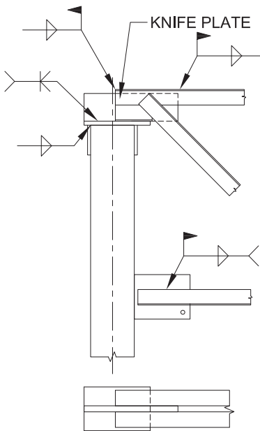
Detail "A"
